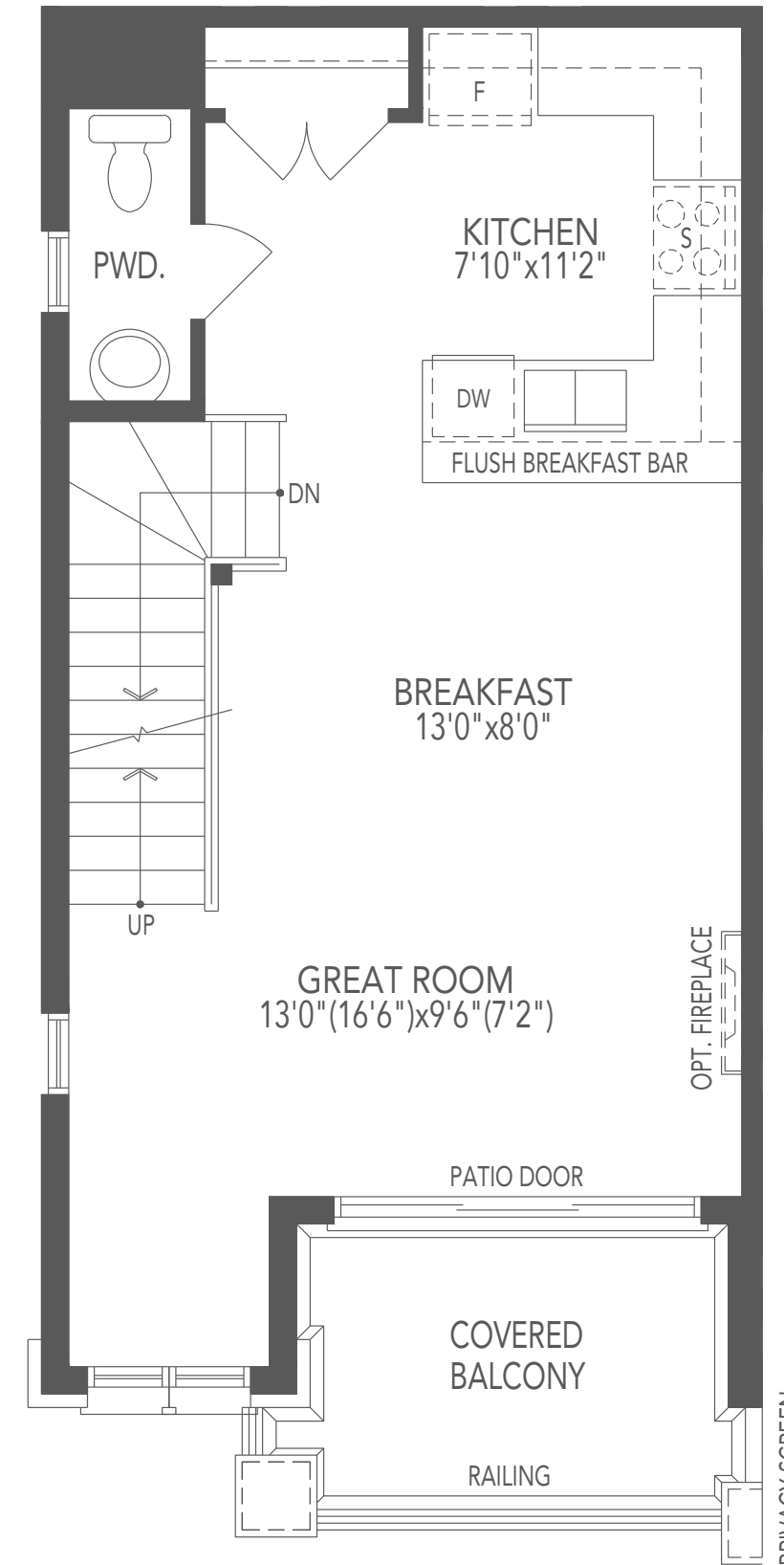
MAIN LEVEL ELEV. B1
