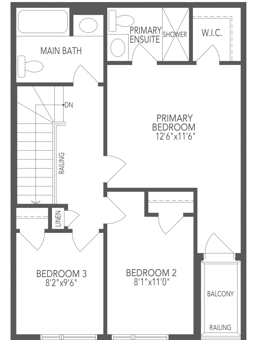
UPPER LEVEL ELEV. A1/A2
