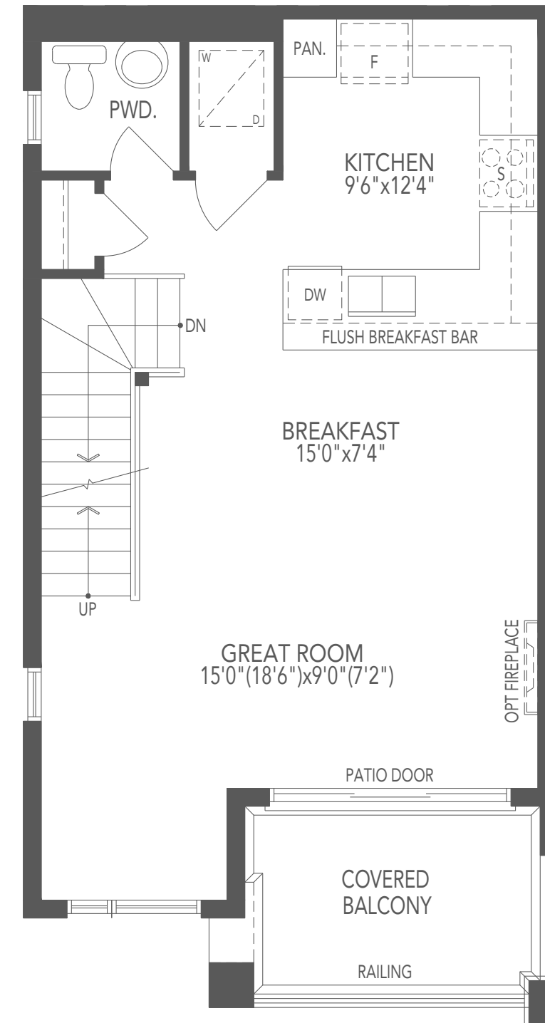
MAIN LEVEL ELEV. A1
