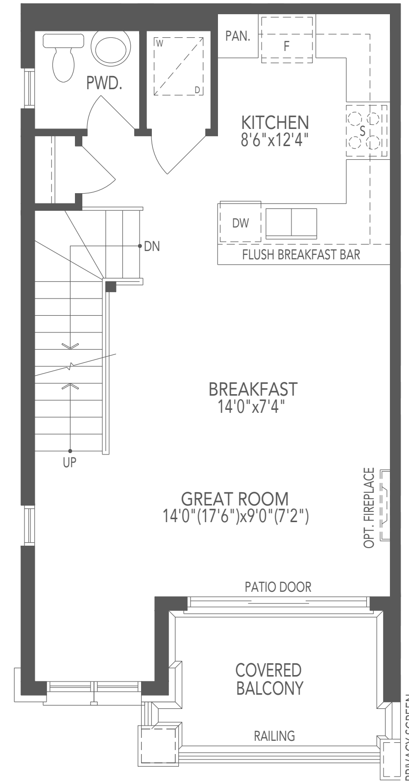
MAIN LEVEL ELEV. A1
